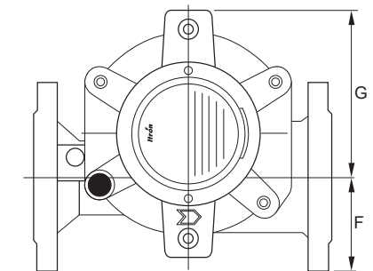
DN 50 upto 150 (flanged)
