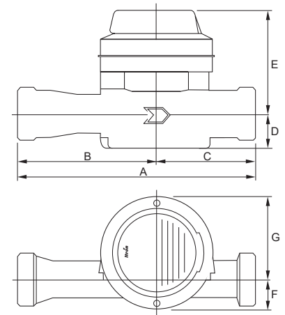
DN 40 and 50 (threaded)
